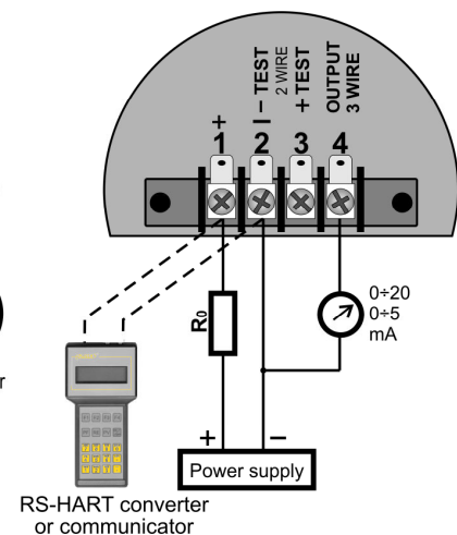
Version: APC-2000ALE with 0...5 or 0...20mA output signal
