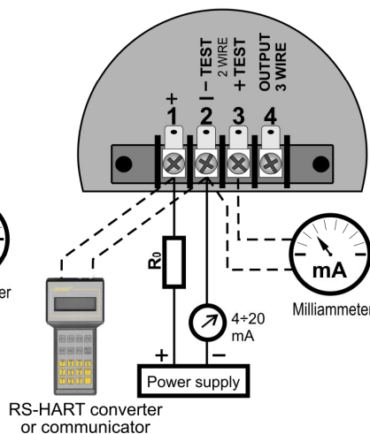
Version: APC-2000ALE with 4...20mA output signal
